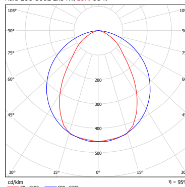
Aura ECO 3001 2x54W, LOR: 95 %
