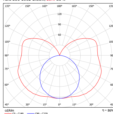
Aura ECO 1002 1x58W, LOR: 86 %
