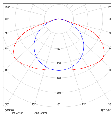
Aura ECO 1502 1x55W, LOR: 56 %
