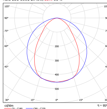
Aura ECO 3001 2x49W, LOR: 95 %
