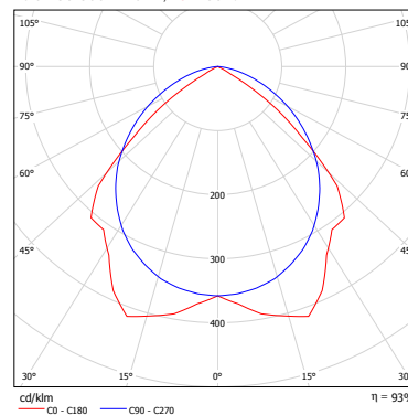
Aura ECO 3004 1x54W, LOR: 93 %
