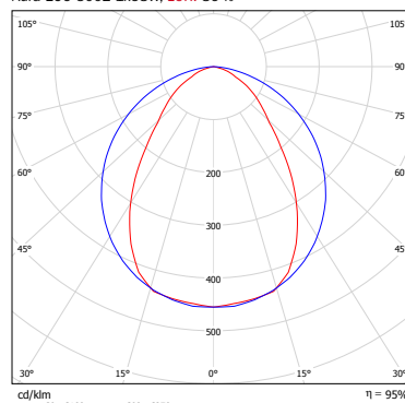
Aura ECO 3002 1x58W, LOR: 86 %
