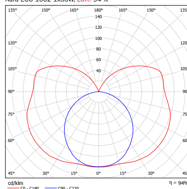
Aura ECO 1002 1x36W, LOR: 94 %
